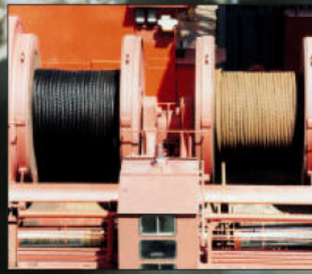
Lubricated with Masto. Unlubricated.
